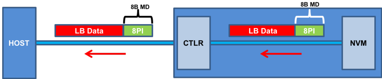
Figure 133: Read 16b Guard Command Protection Information Processing
