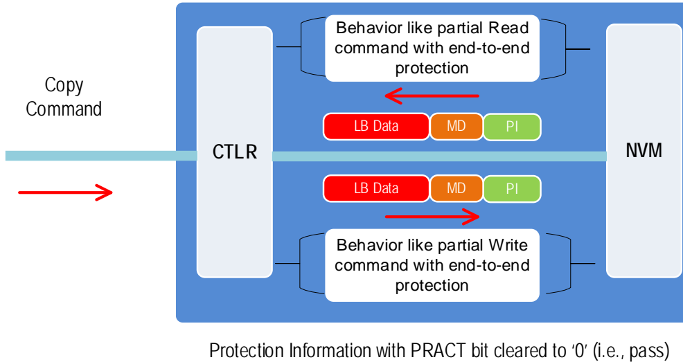
Figure 135: Protection Information Processing for Copy
