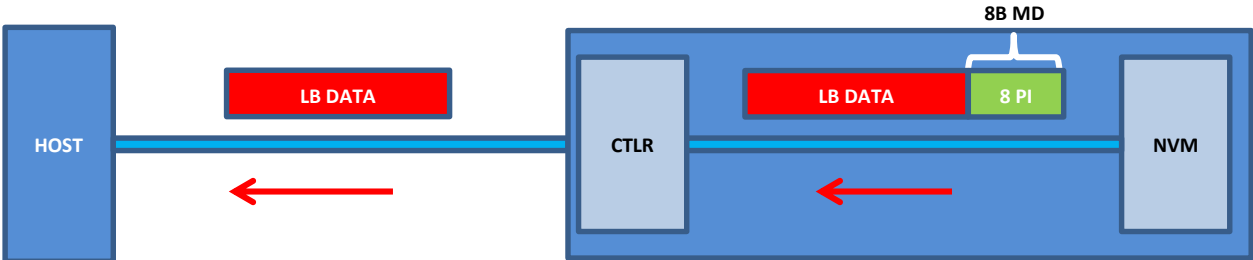
c) MD=8, PI, PRACT=1: Metadata not resident in host buffer
