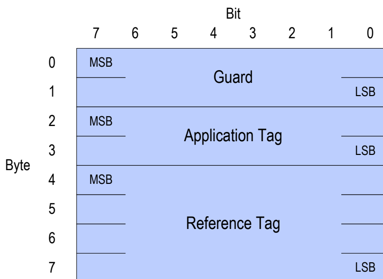
Figure 214: Protection Information Format
