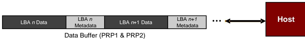
Figure 212: Metadata – Contiguous with LBA Data, Forming Extended LBA
