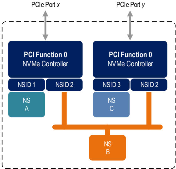
Figure 5: NVM Subsystem with Two Controllers and Two Ports
