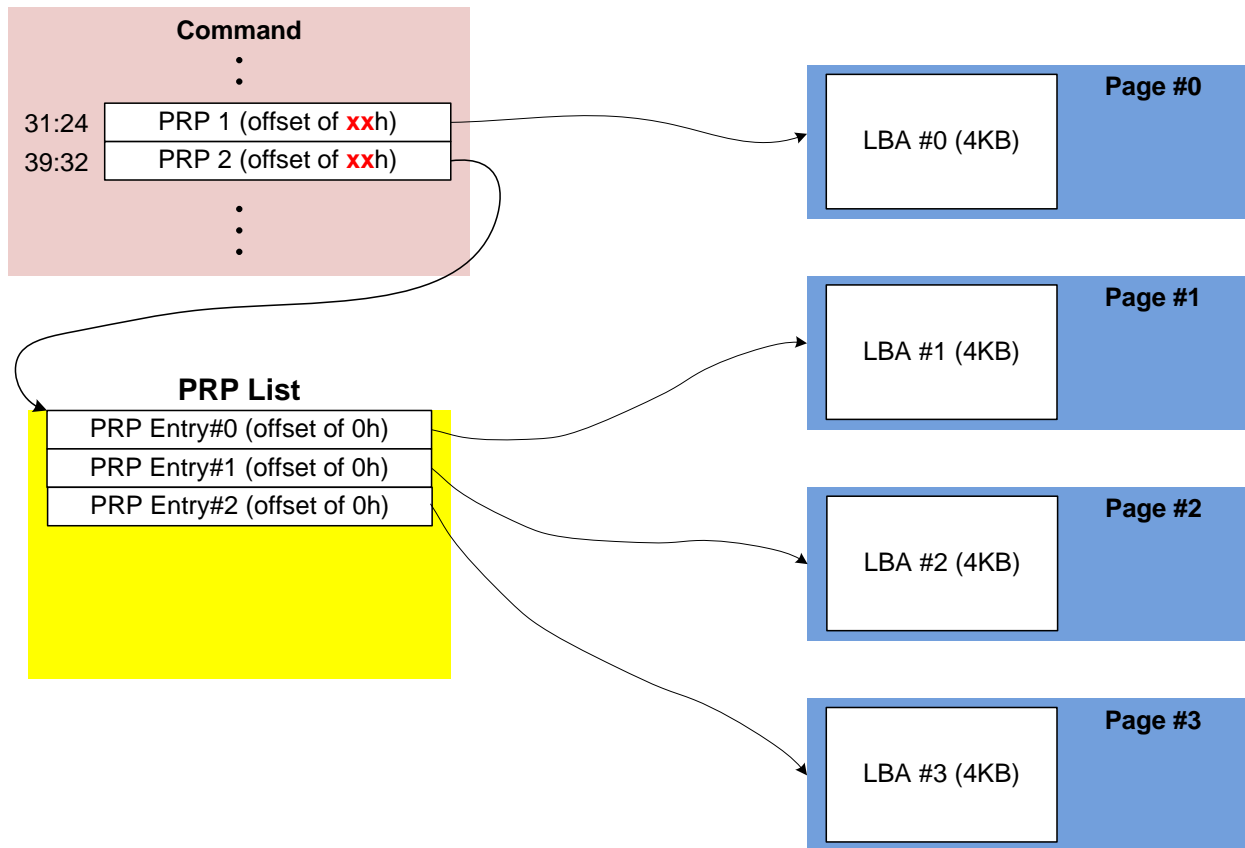
Figure 211: PRP List Describing Data to Compare
