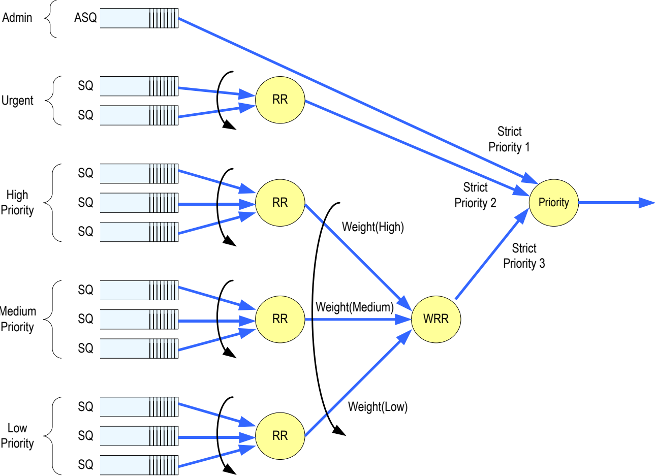
Figure 39: Weighted Round Robin with Urgent Priority Class Arbitration
