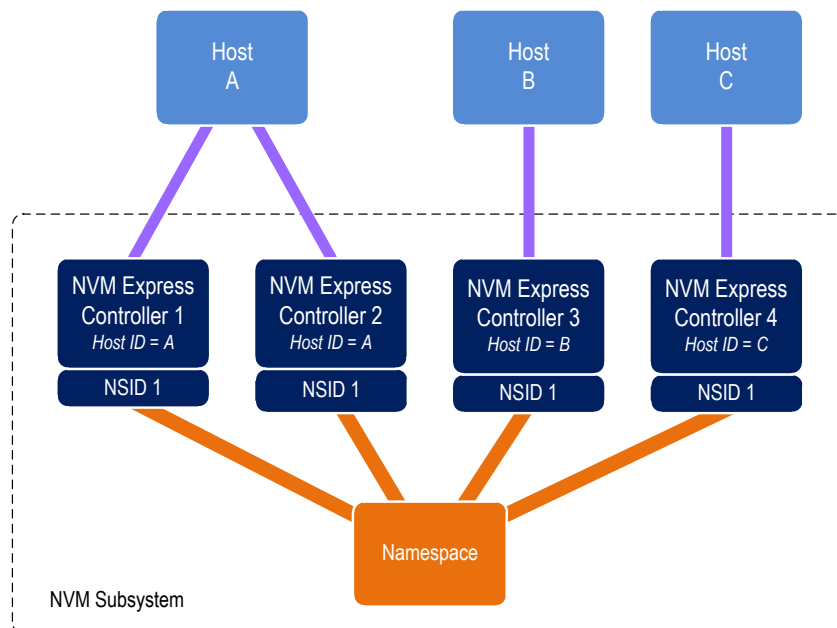
Figure 221: Example Multi-Host System
