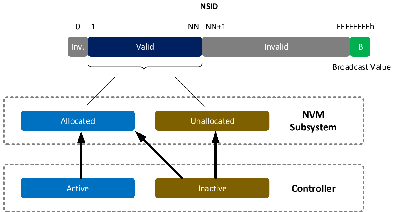
Figure 150: NSID Types
