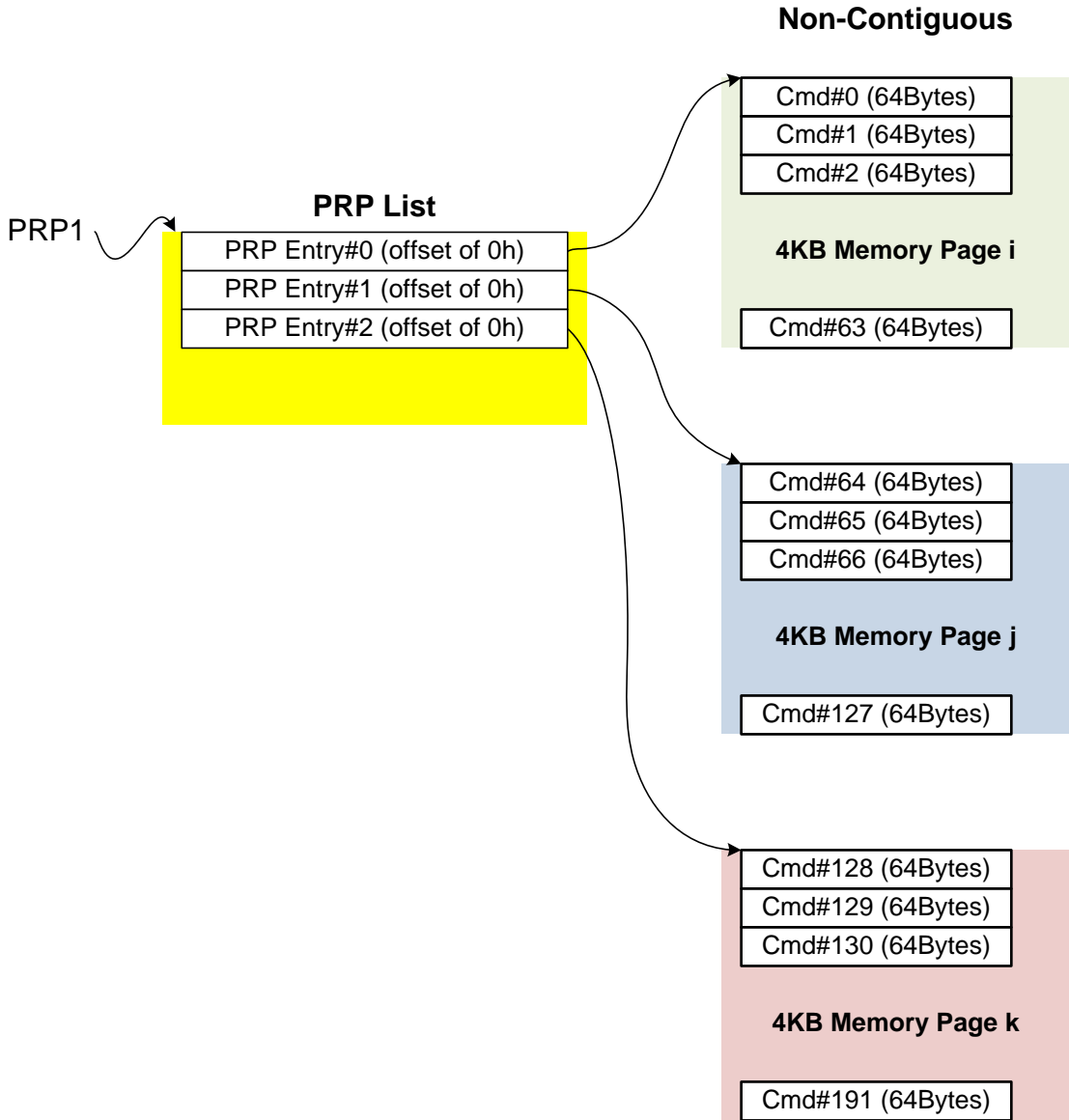
Figure 210: PRP List Describing I/O Submission Queue
