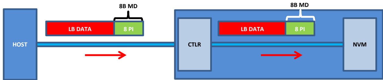
Figure 215: Write Command Protection Information Processing
