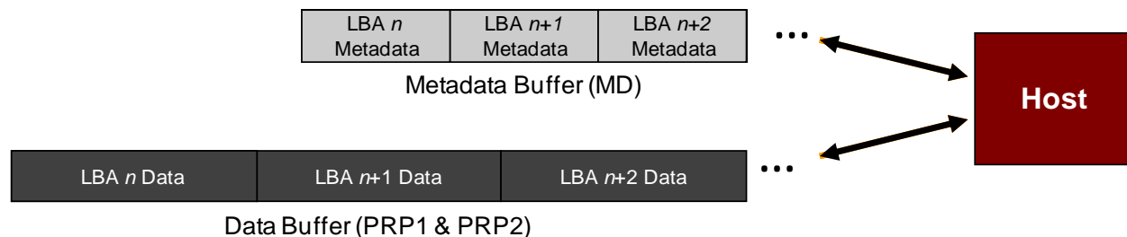
Figure 213: Metadata – Transferred as Separate Buffer
