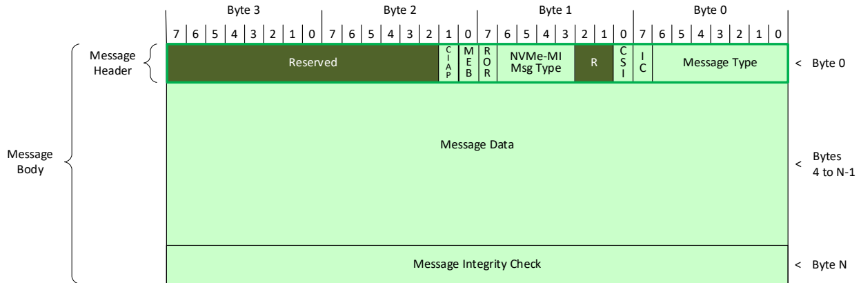
Figure 18: NVMe-MI Message
