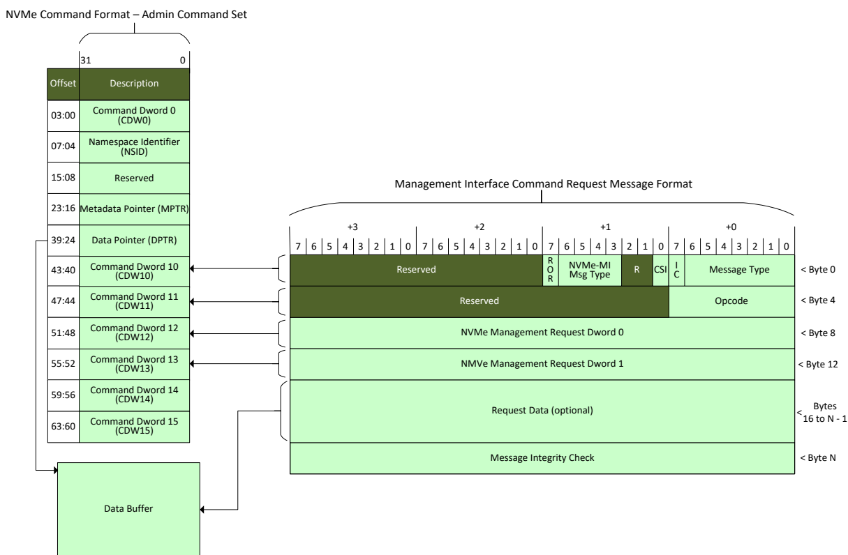
Figure 42: NVMe-MI Send Command Request Message to NVMe Admin Command SQE Mapping Diagram
