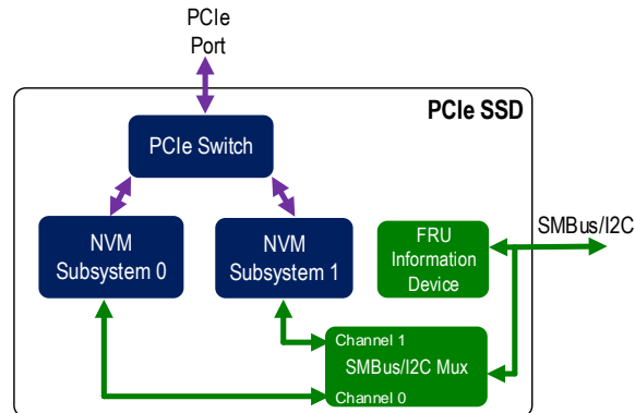
Figure 7: NVMe Storage Device with two NVMe Subsystems and an SMBus/I2C Mux
