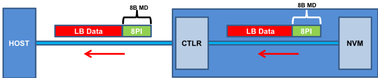
Figure 255: Read Command Protection Information Processing
