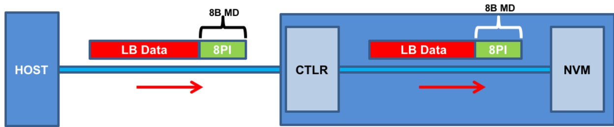
Figure 254: Write Command Protection Information Processing
