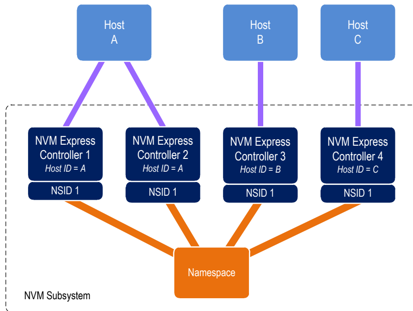
Figure 262: Example Multi-Host System
