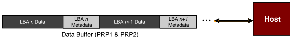
Figure 251: Metadata – Contiguous with LBA Data, Forming Extended LBA
