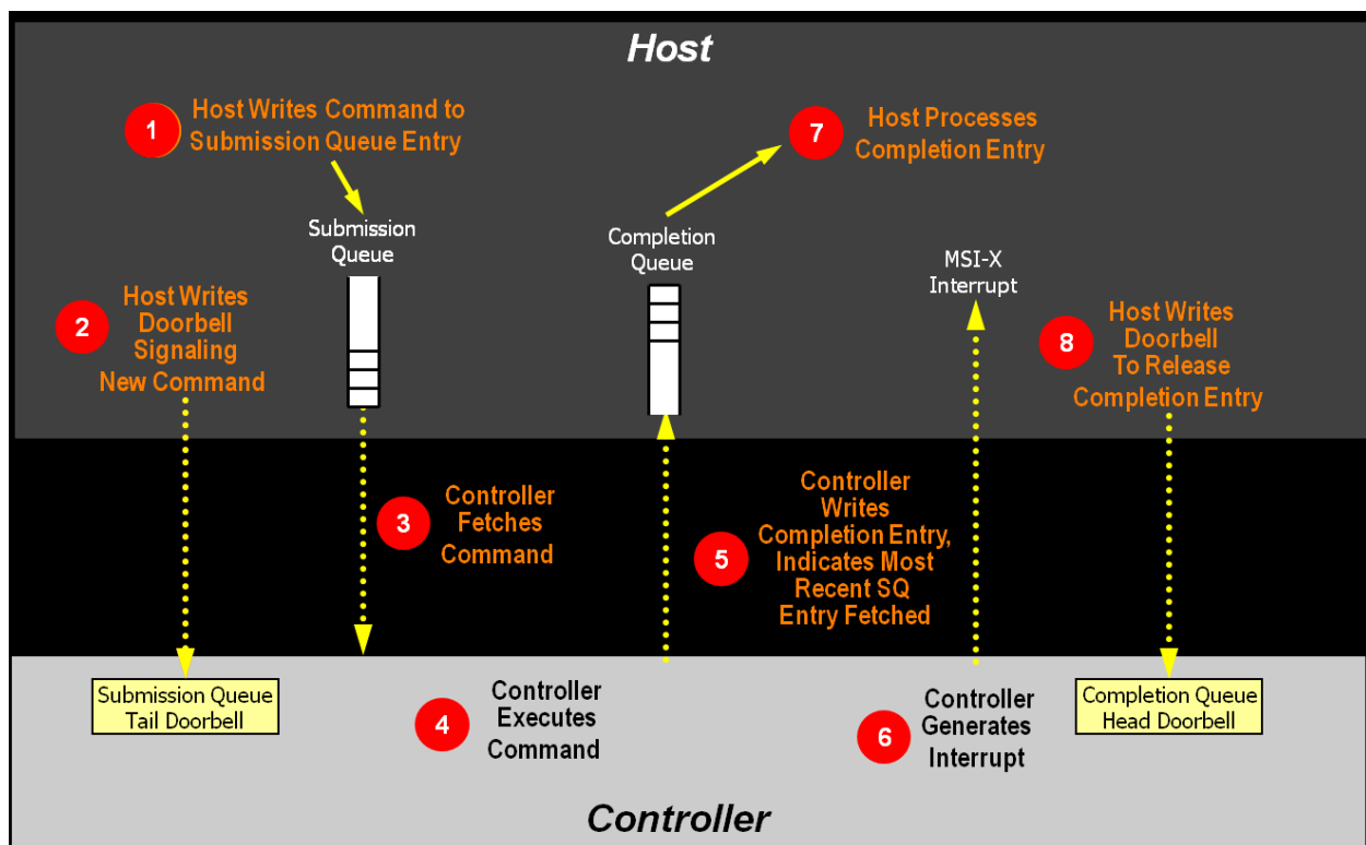
Figure 247: Command Processing
