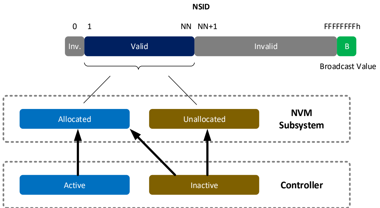
Figure 185: NSID Types
