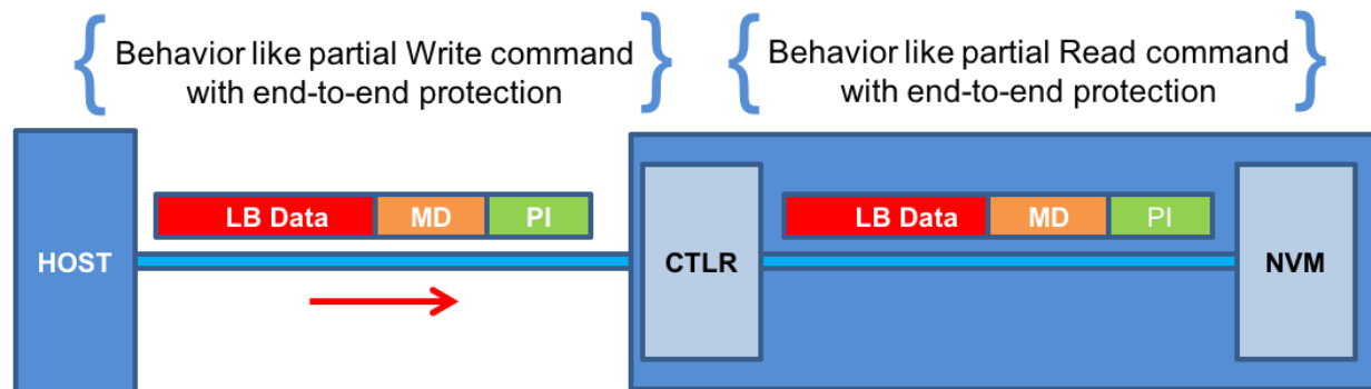
Figure 256: Protection Information Processing for Compare
