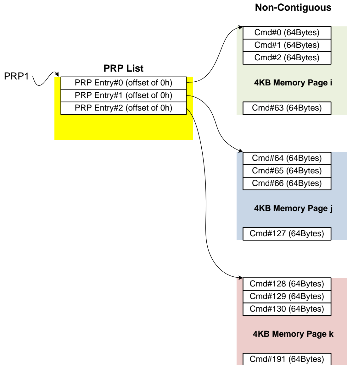
Figure 248: PRP List Describing I/O Submission Queue
