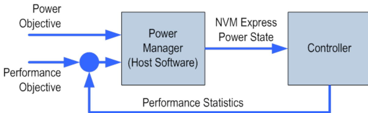
Figure 257: Dynamic Power Management
