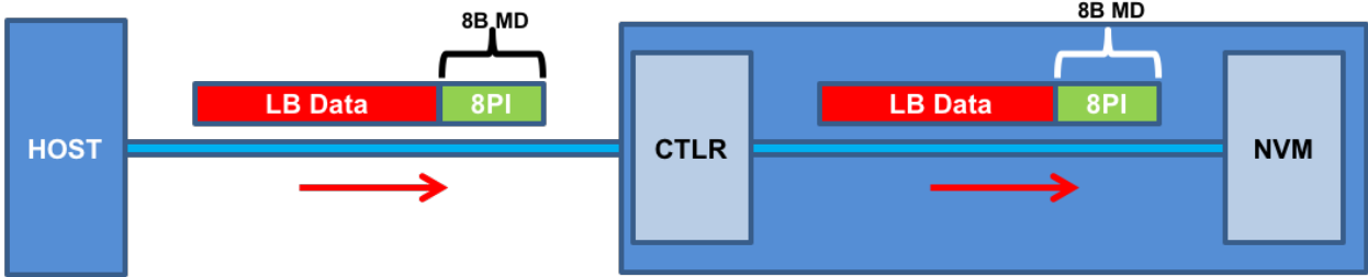
a) MD=8, PI, PRACT=0: Metadata remains same size in NVM and host buffer
