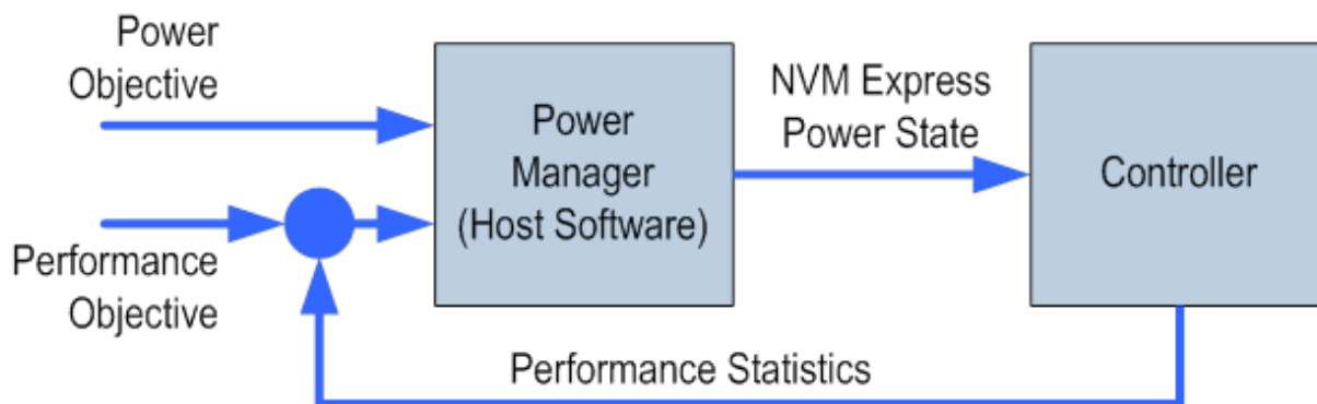
Figure 255: Dynamic Power Management
