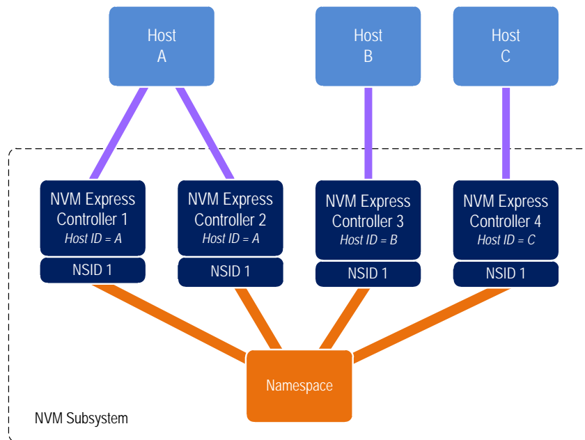
Figure 260: Example Multi-Host System
