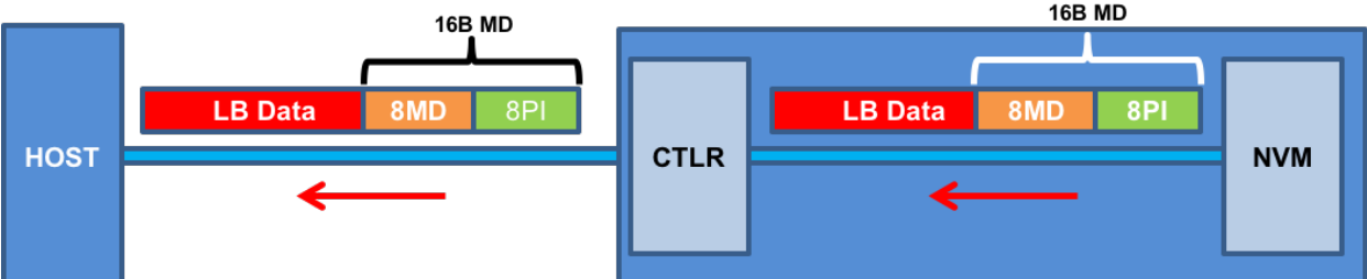
d) MD>8 (e.g., 16), PI, PRACT=1: Metadata remains same size in NVM and host buffer
