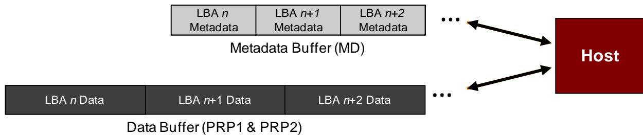
Figure 250: Metadata – Transferred as Separate Buffer
