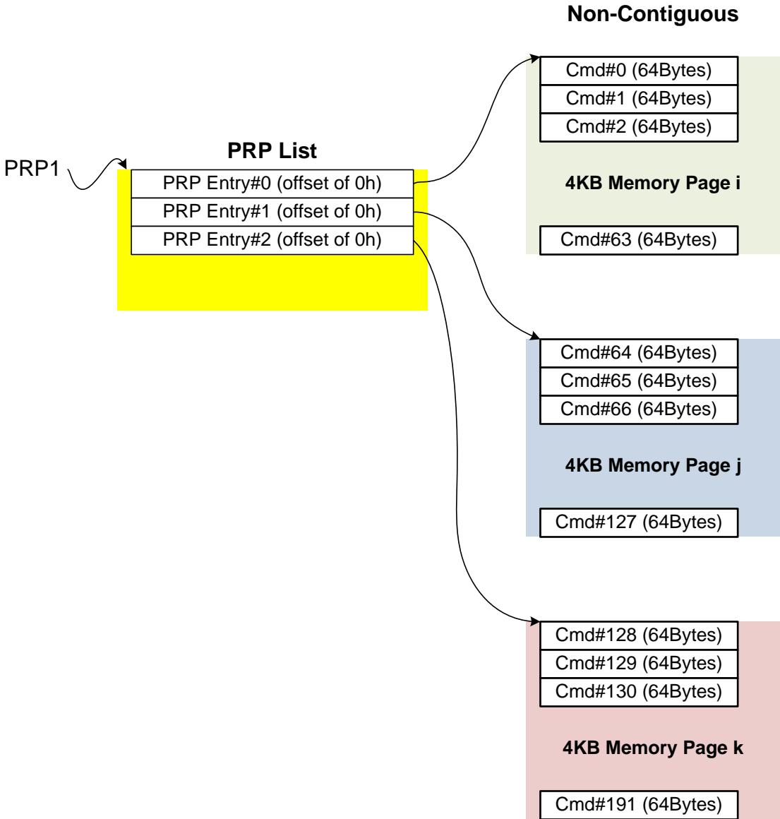
Figure 246: PRP List Describing I/O Submission Queue
