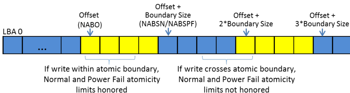
Figure 189: Atomic Boundaries Example
