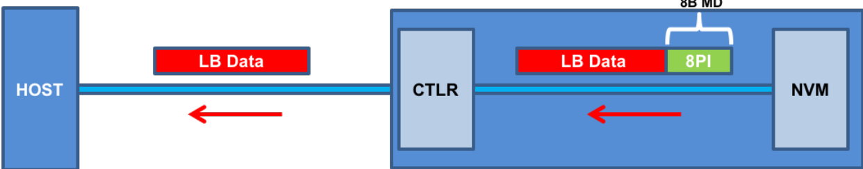
c) MD=8, PI, PRACT=1: Metadata not resident in host buffer
