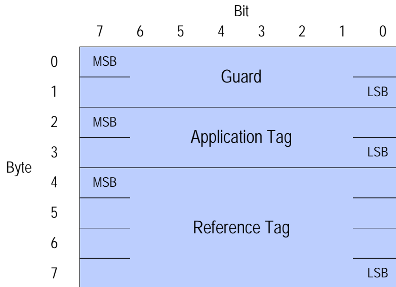
Figure 251: Protection Information Format
