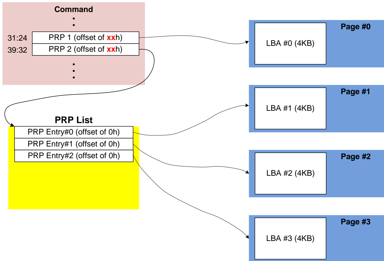
Figure 247: PRP List Describing Data to Compare
