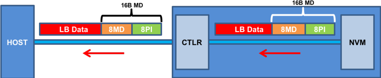
b) MD>8 (e.g., 16), PI, PRACT=0: Metadata remains same size in NVM and host buffer
