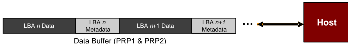
Figure 249: Metadata – Contiguous with LBA Data, Forming Extended LBA
