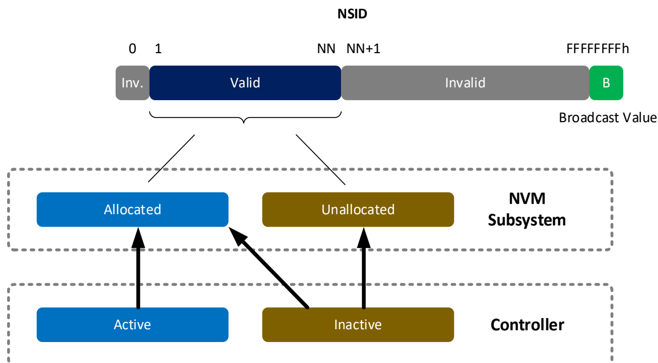
Figure 183: NSID Types
