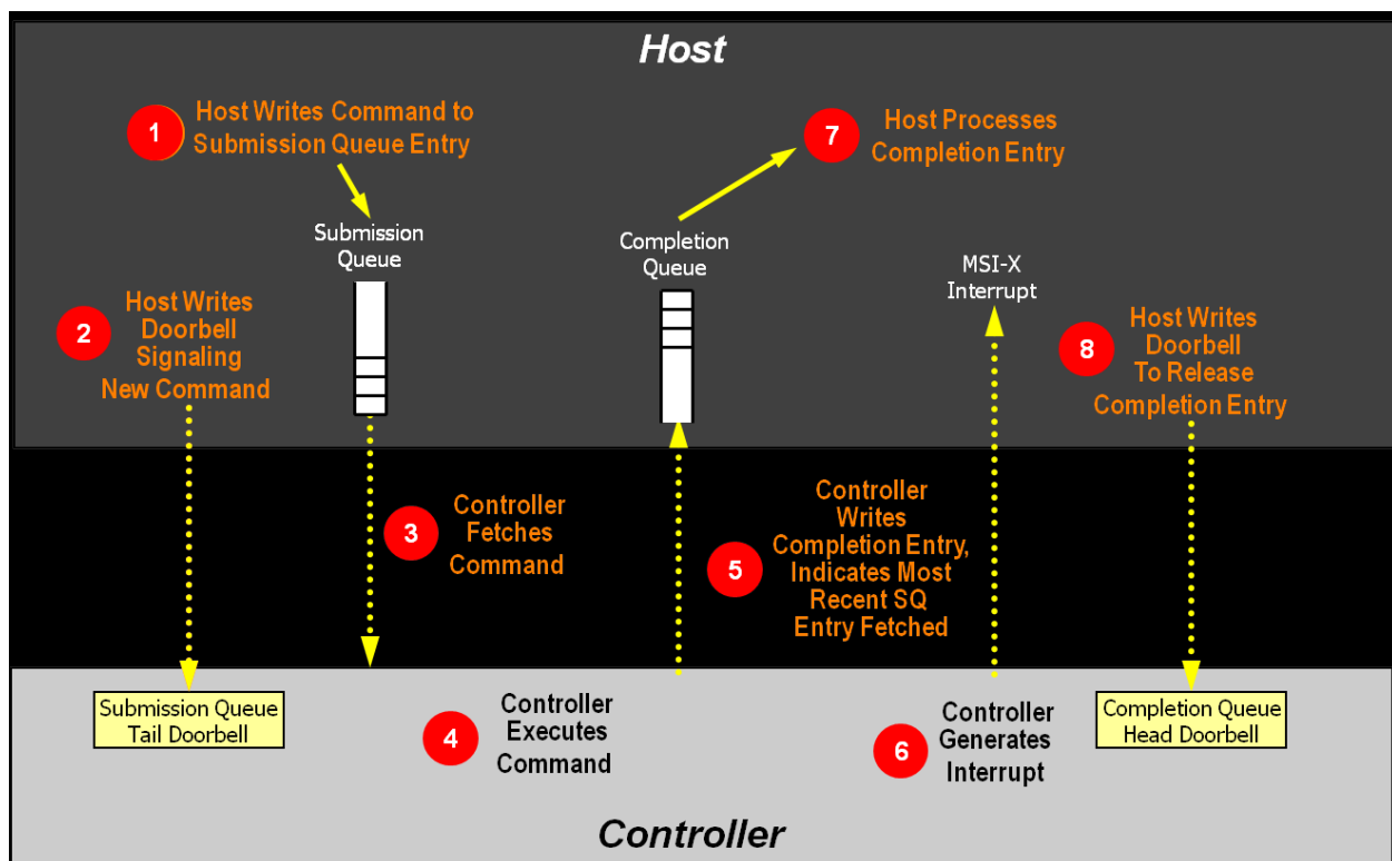
Figure 245: Command Processing
