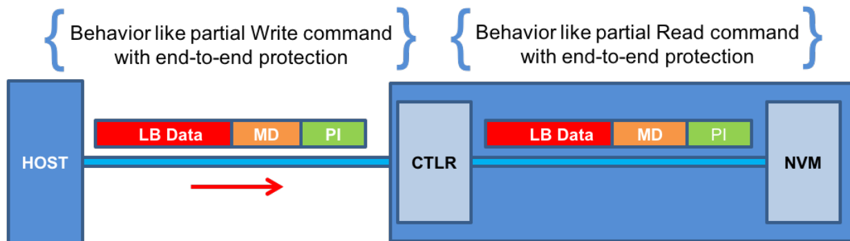
Figure 254: Protection Information Processing for Compare
