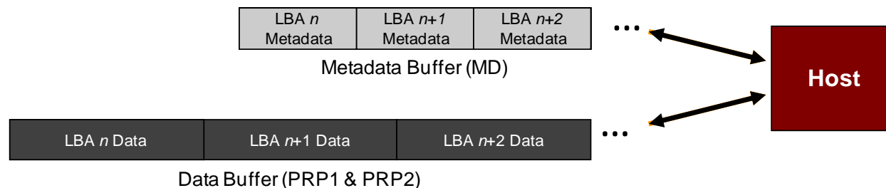
Figure 212: Metadata – Transferred as Separate Buffer
