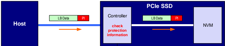
(c) Protection Information with PRACT bit cleared to '0' (i.e., pass)
