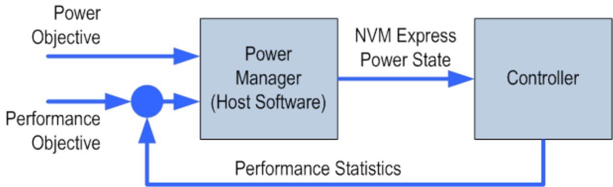
Figure 217: Dynamic Power Management
