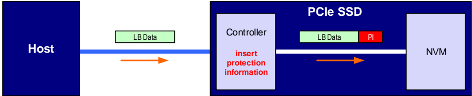
(d) Protection Information with PRACT bit set to '1' (i.e., insert)
