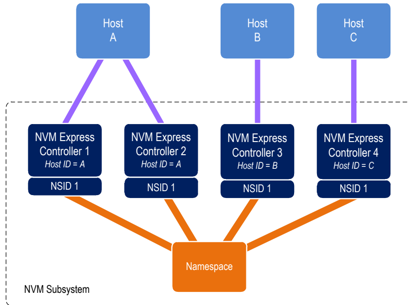
Figure 220: Example Multi-Host System
