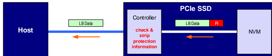
(d) Protection Information with PRACT bit set to '1' (i.e., strip)
