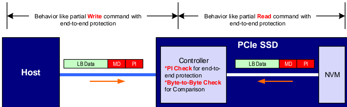
Figure 215: Protection Information Processing for Compare
