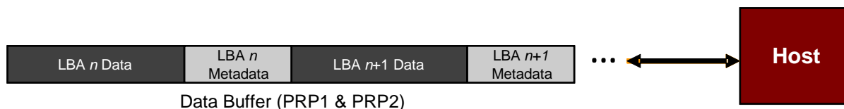
Figure 211: Metadata – Contiguous with LBA Data, Forming Extended LBA
