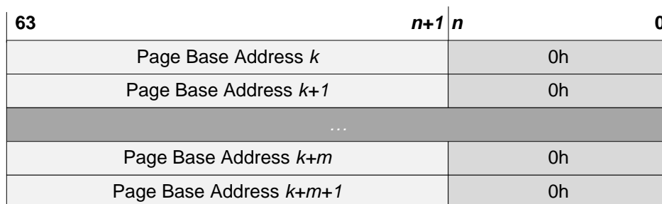
Figure 11: PRP List Layout
