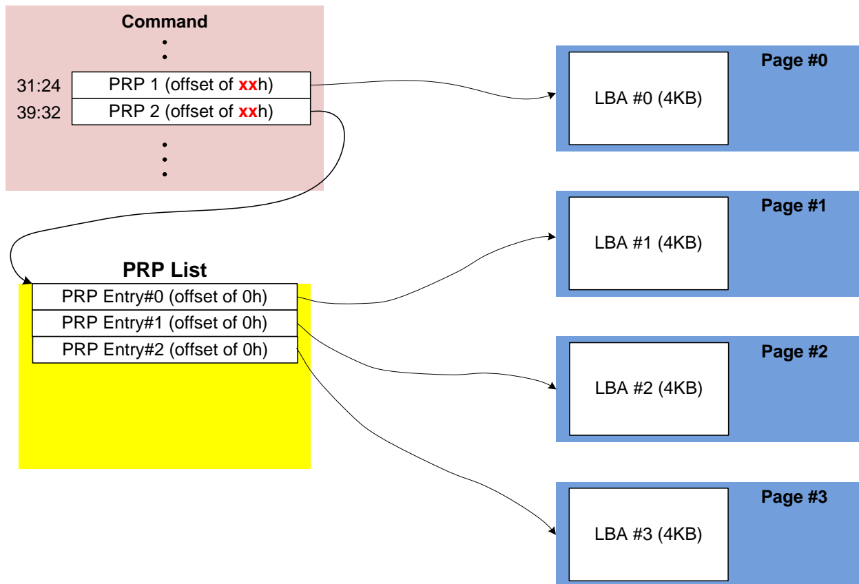
Figure 139: PRP List Describing Data to Compare
