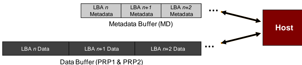
Figure 141: Metadata – Transferred as Separate Buffer
