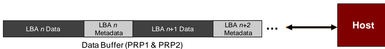
Figure 140: Metadata – Contiguous with LBA Data, Forming Extended LBA
