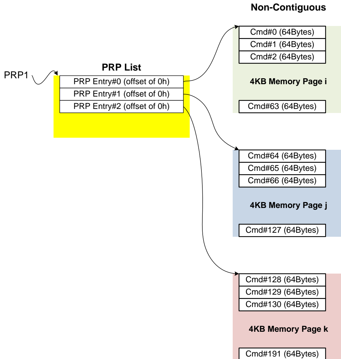
Figure 138: PRP List Describing I/O Submission Queue
